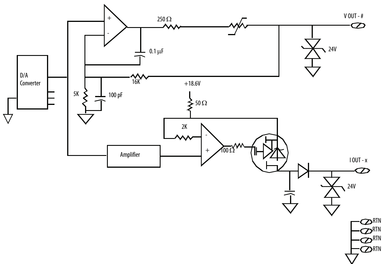
Figure 23 - 1756-OF8H Output Circuit Diagram
