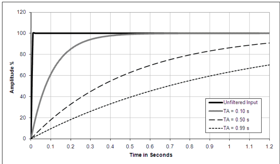
Figure 16 - Filter Response
