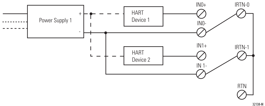
Figure 7 - Single Power Supply with Multiple HART Devices
