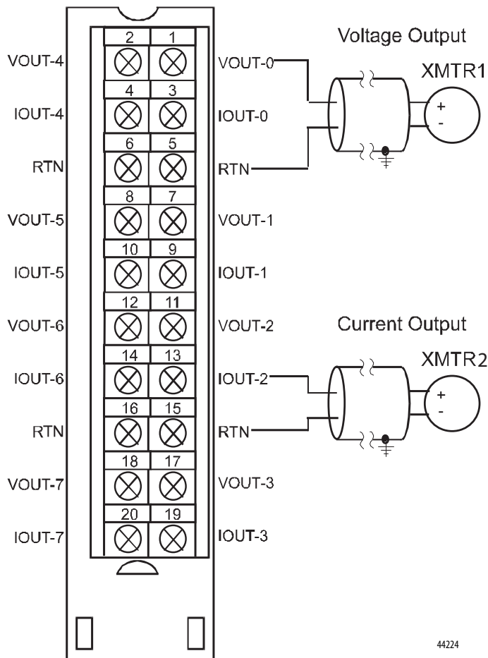
Figure 22 - Wiring Diagram for the 1756-OF8H Module
