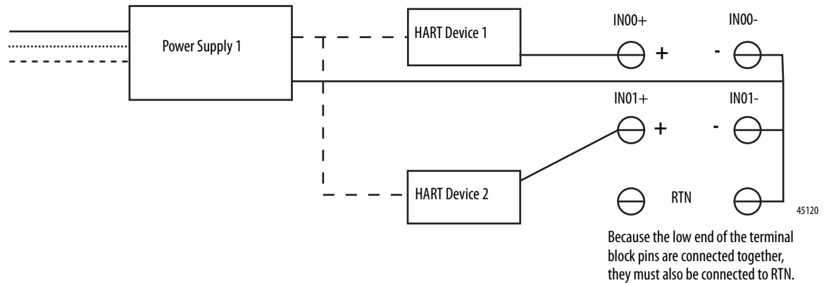
Figure 18 - Single Power Supply with Multiple HART Devices
