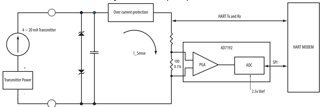
Figure 14 - 1756-IF8IH Simplified Input Circuit
