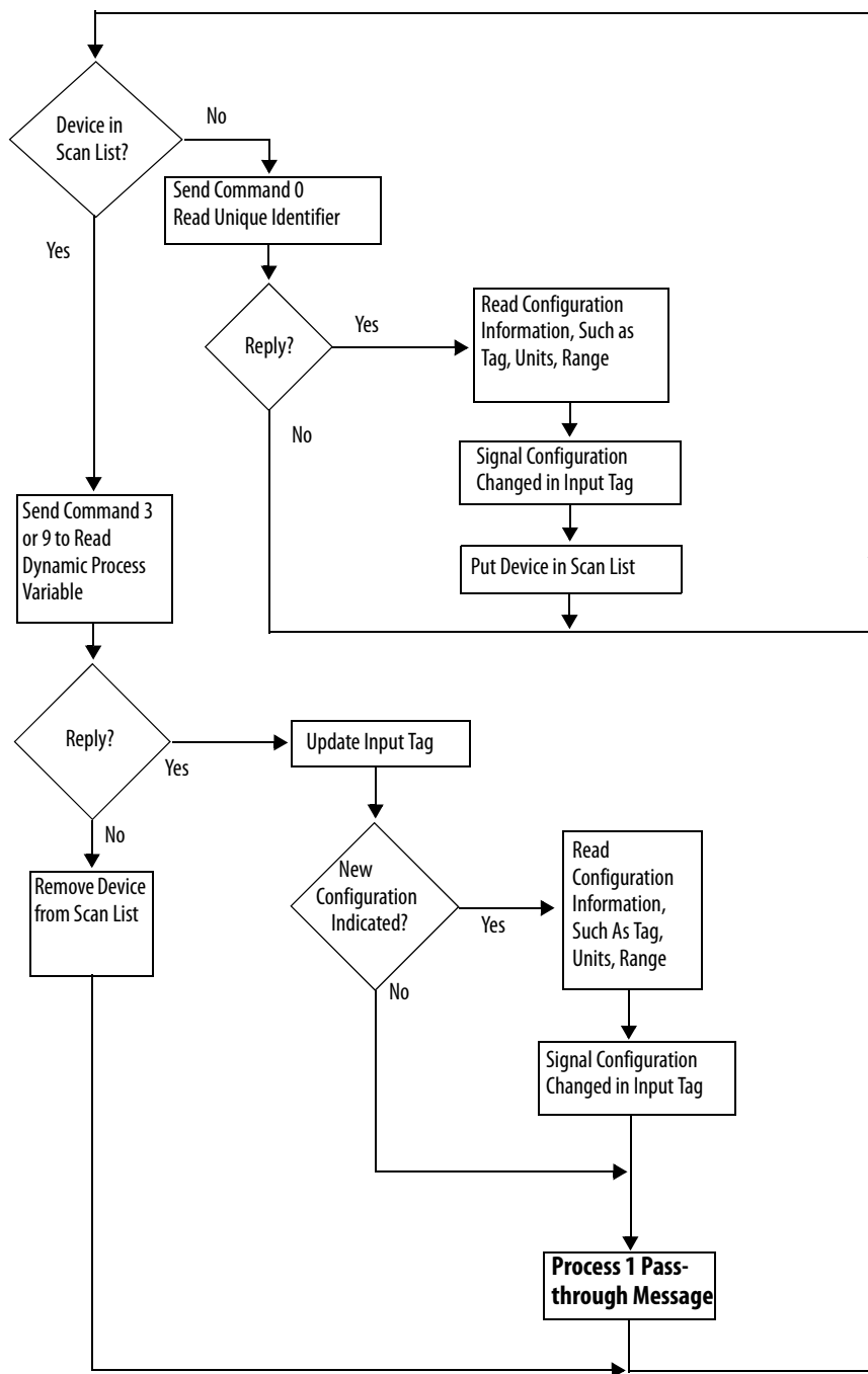
Figure 29 - 1756-IF8IH, 1756-OF8IH, and 1756-IF16H Flow Chart
