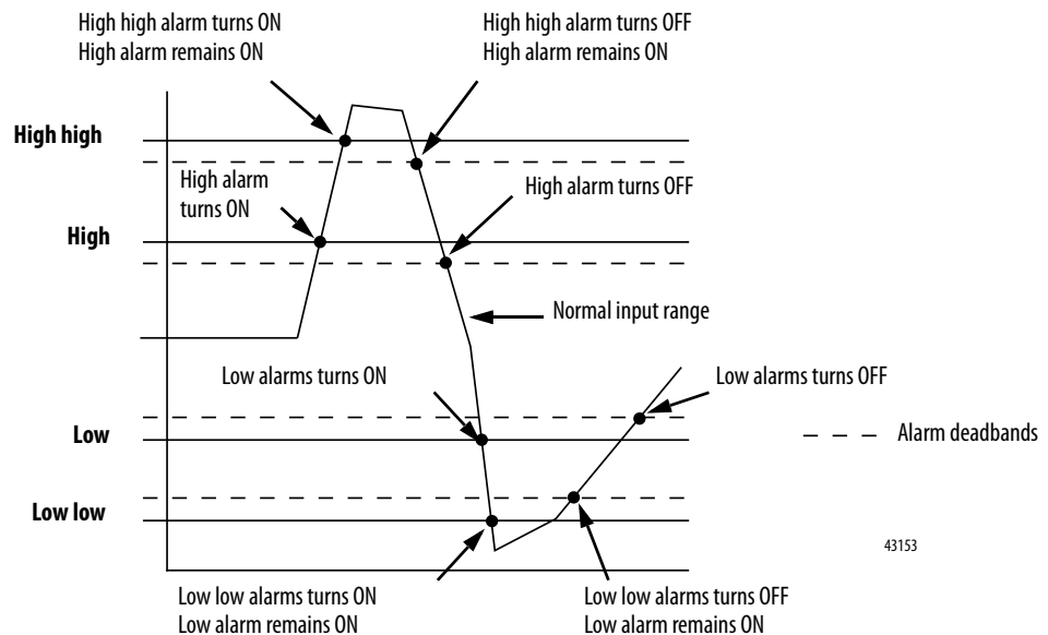
Figure 5 - Input Data That Sets Each of the Alarms
