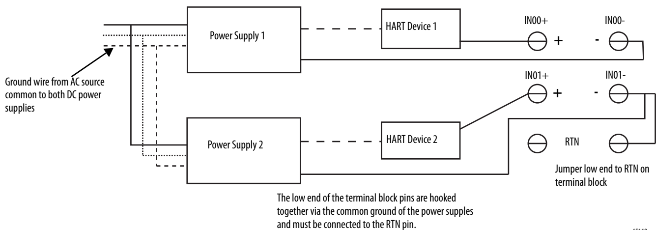
Figure 19 - Multiple Power Supplies with a Common Ground
