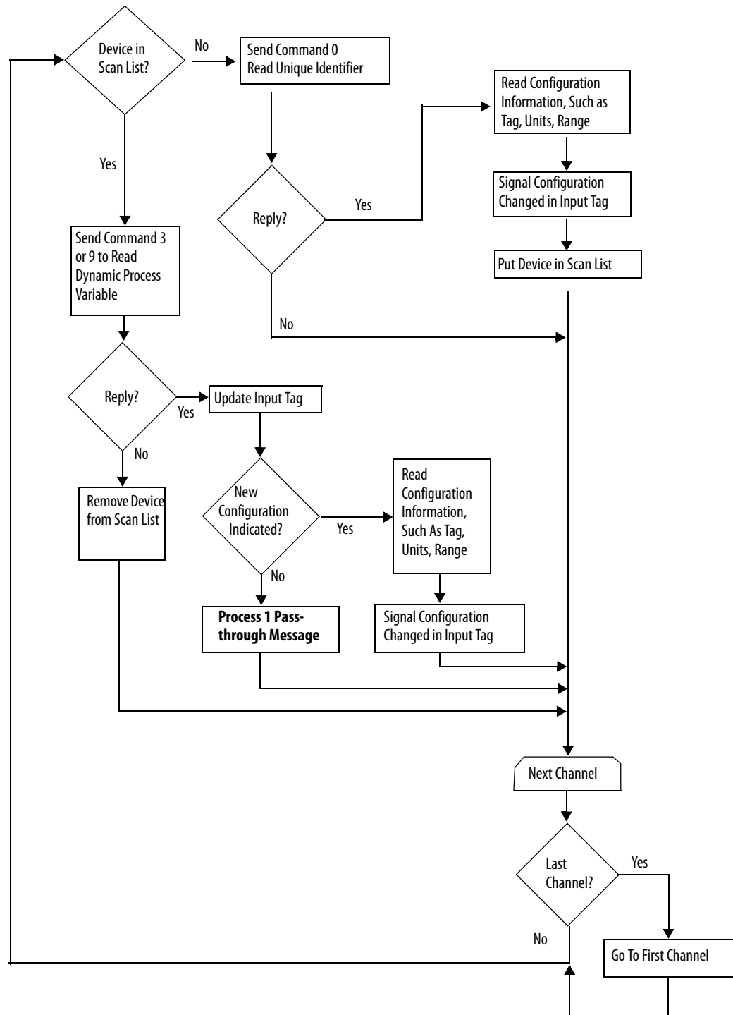
Figure 28 - 1756-IF8H and 1756-OF8H Flow Chart.
