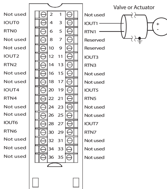
Figure 24 - Wiring Diagram for the 1756-OF8IH Module
