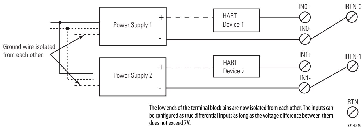
Figure 9 - Power Supplies with Isolated Grounds
