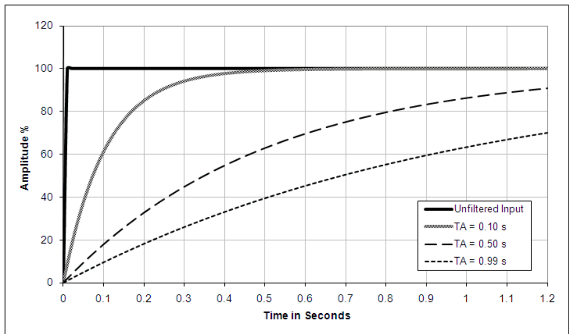
Figure 12 - Filter Response
