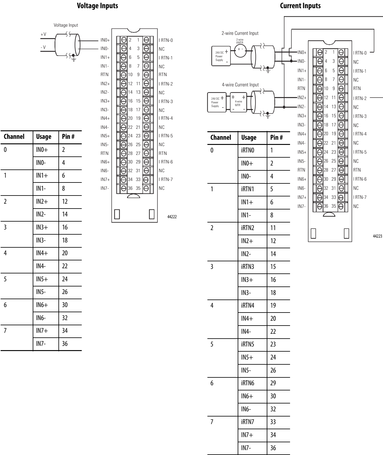
Figure 6 - 1756-IF8H Voltage and Current Inputs
