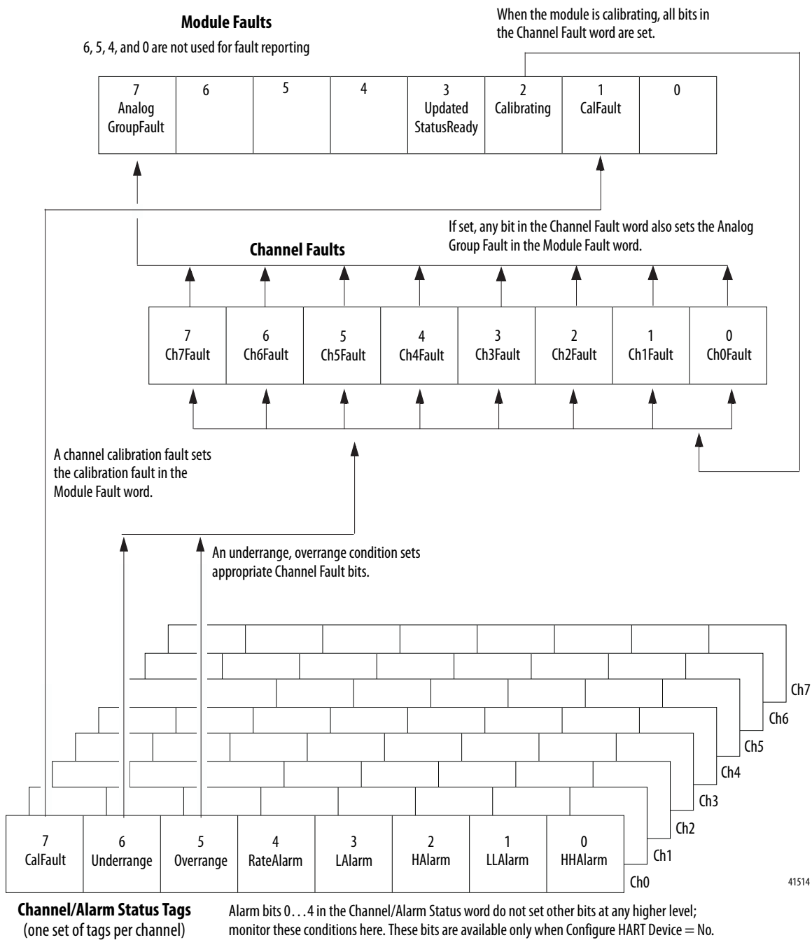
Figure 15 - 1756-IF8IH Module Fault Reporting
