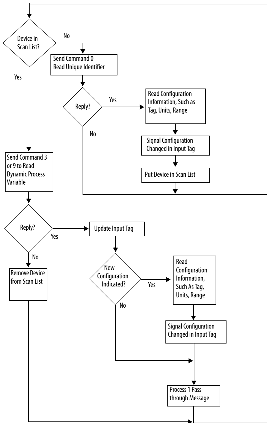
Figure 27 - 1756-IF8IH, 1756-OF8IH, and 1756-IF16H Flow Chart
