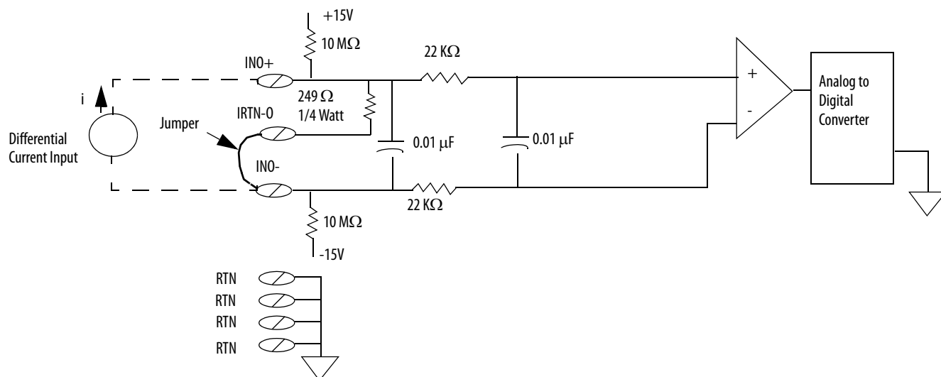
Figure 10 - Simplified 1756-IF8H Current Input Circuit
