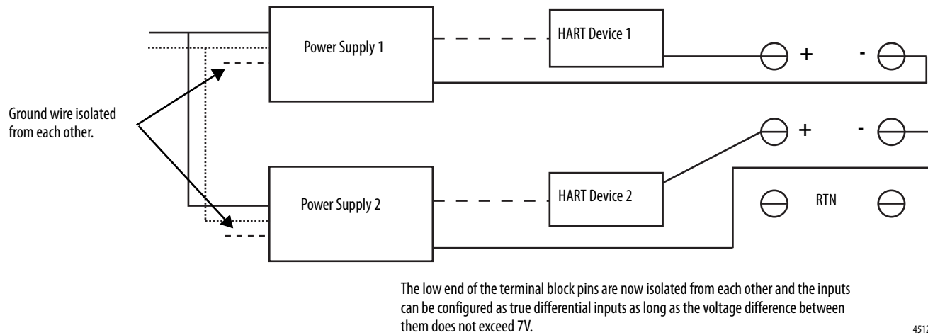
Figure 20 - Power Supplies with Isolated Grounds
