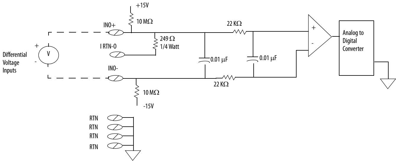
Figure 11 - Simplified 1756-IF8H Voltage Input Circuit
