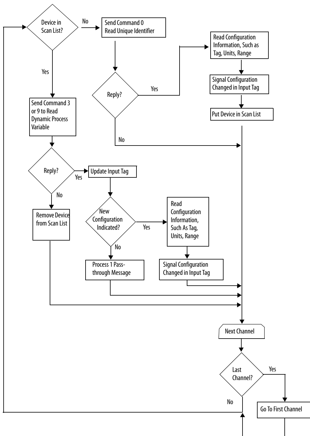
Figure 26 - 1756-IF8H and 1756-OF8H Flow Chart
