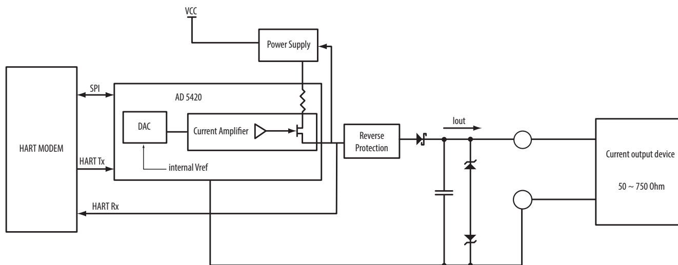
Figure 25 - 1756-OF8IH Output Circuit Diagram
