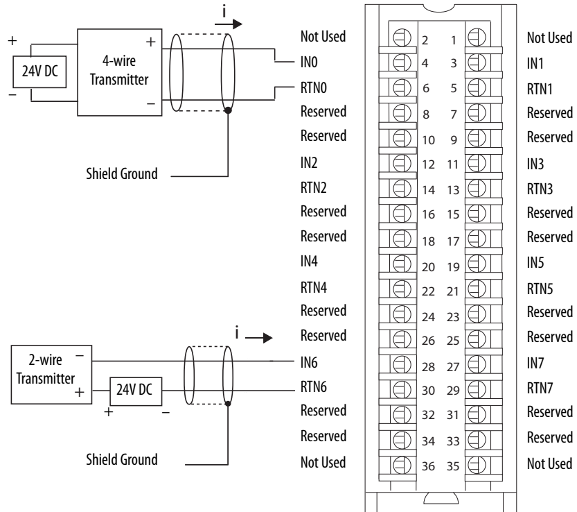
Figure 13 - 1756-IF8IH Wiring Diagram
