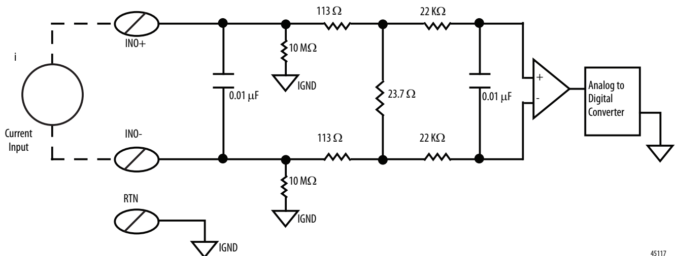
Figure 21 - 1756-IF16H Simplified Current Input Circuit
