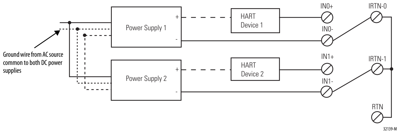
Figure 8 - Multiple Power Supplies with a Common Ground
